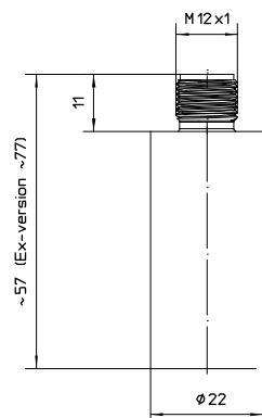
circular connector with screw cap M12x1 degree of protection IP65 / IP67
