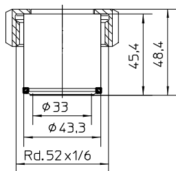
HYGENIC-Tubus * Ø43,3 with screwing DN25/PN40
