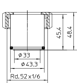
HYGENIC-Tubus * Ø43.3 with screwing DN25/PN40
